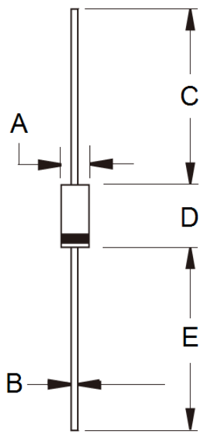
DO-204AC (DO-15)
