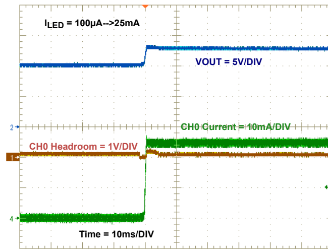
FIGURE 13. TRANSIENT RESPONSE (LED CURRENT CHANGES from 100μA to 25mA)
