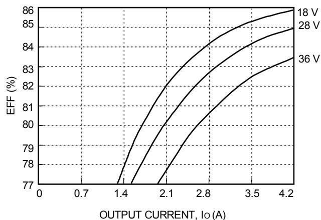
Figure 7. Typical JC050B Converter Efficiency vs. Output Current at Room Temperature
