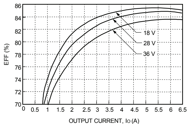
Figure 8. Typical JC075B Converter Efficiency vs. Output Current at Room Temperature
