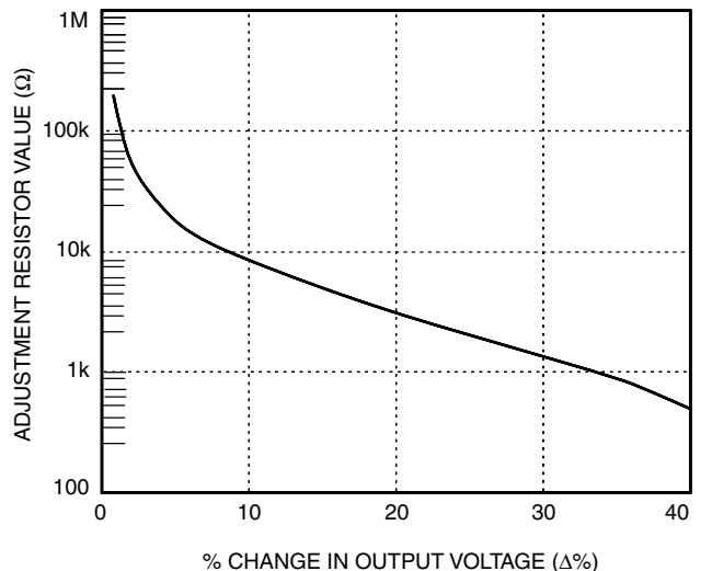
Figure 17. Resistor Selection for Decreased Output Voltage
