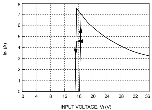
Figure 3. Typical JC100B Input Characteristics at Room Temperature, I_o = Full Load
