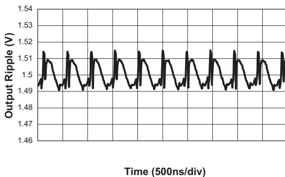
Output Ripple ( V_{IN} = 3.6V ; V_{OUT} = 1.5V ; I_{OUT} = 300mA )
