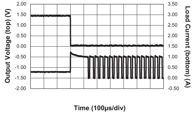
Short Circuit ( V_{IN} = 3.6V ; V_{OUT} = 1.5V )
