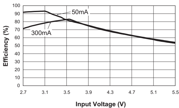
Efficiency vs. Input Voltage ( V_{OUT} = 1.5V )
