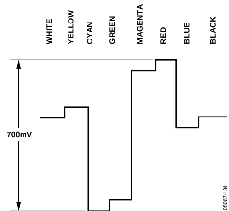
Figure 134. Pr Levels—PAL
