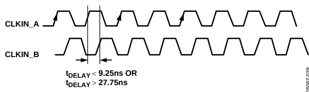
Figure 53. Clock Phase with Two Input Clocks
