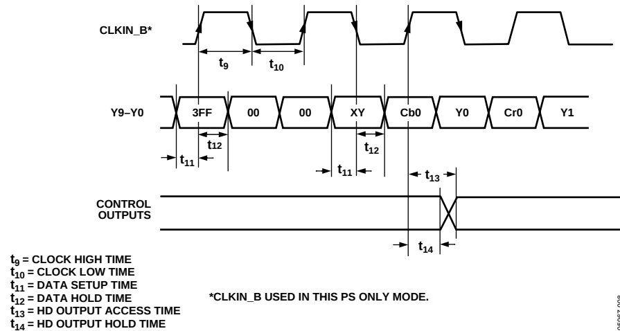
Figure 8. PS Only 4:2:2 10-Bit Interleaved at 27 MHz EAV/SAV Input Mode (Input Mode 100)
