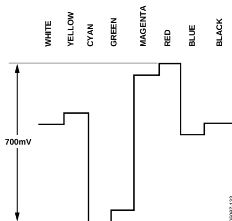
Figure 133. Pr Levels—NTSC
