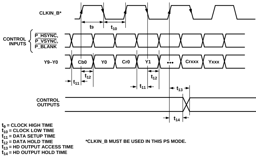
Figure 6. PS 4:2:2 10-Bit Interleaved at 27 MHz \overline{\text{HSYNC}}/\overline{\text{VSYNC}} Input Mode (Input Mode 100)
