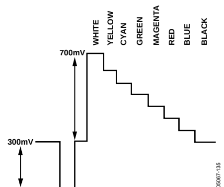
Figure 135. Y Levels—NTSC
