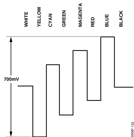
Figure 132. Pb Levels—PAL
