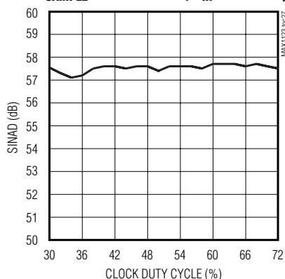
SINAD vs. CLOCK DUTY CYCLE ( f_{IN} = 1.4106MHz , f_{SAMPLE} = 210.0428MHz , A_{IN} = -0.5dBFS )
