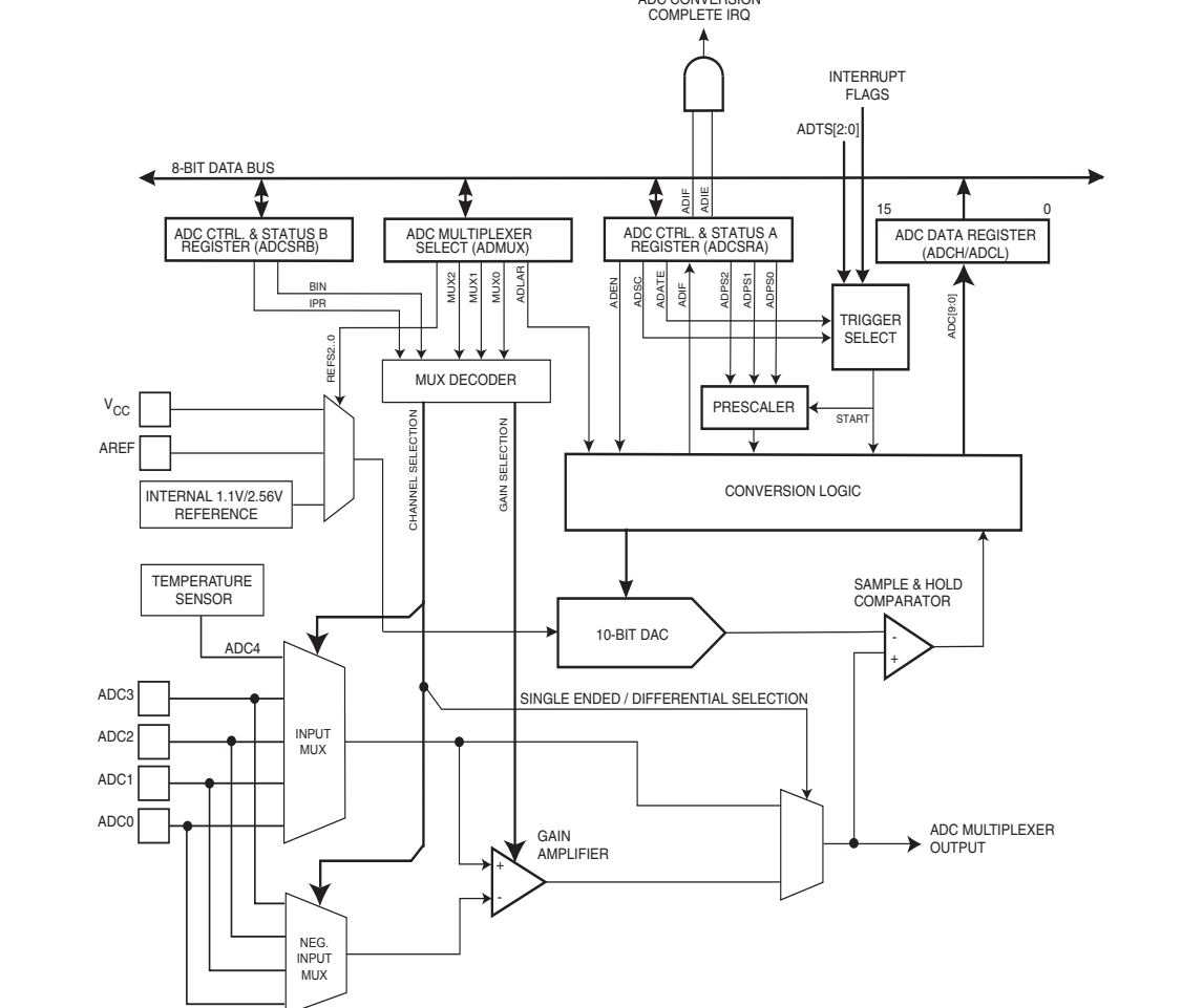
ADC CONVERSION
