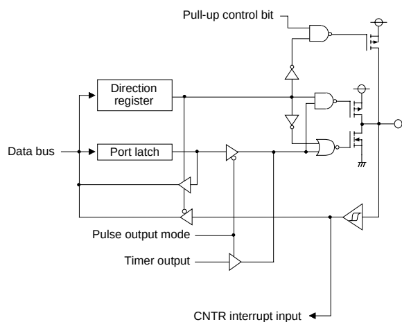
Fig. 14 Port block diagram (3)
