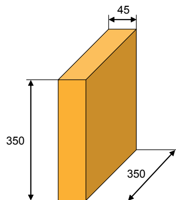
Figure 20. Inner box dimensions for 13" reel
