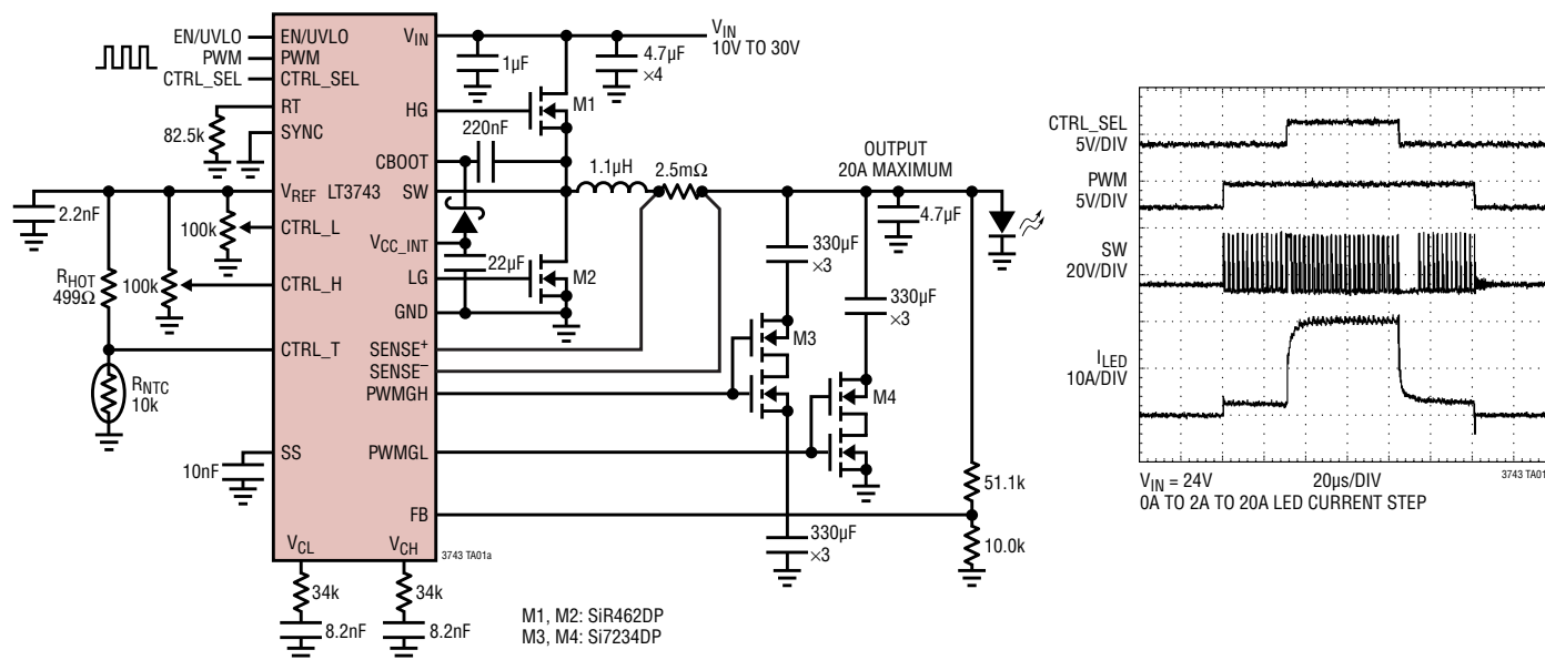
92% Efficient 20A LED Driver
