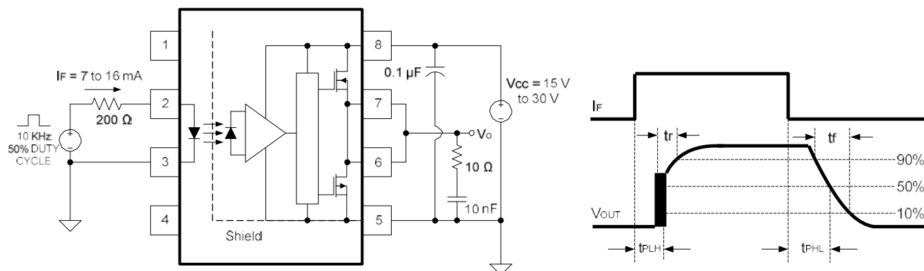
Figure 23 : t_r , t_f , t_{PLH} and t_{PHL} Test Circuit and Waveforms
