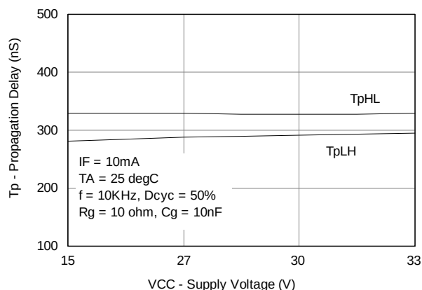
Figure 10: Propagation vs Vcc
