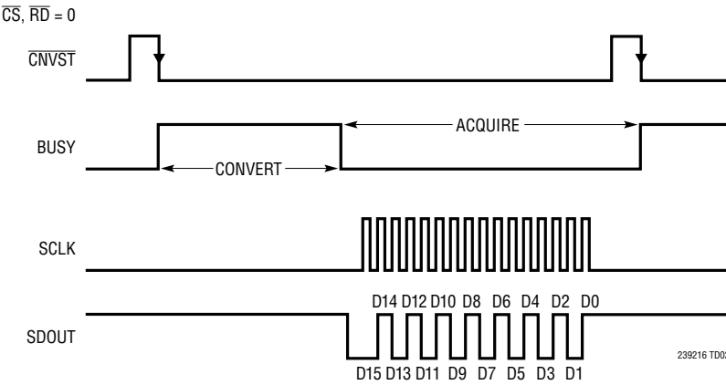
Conversion Timing Using the Serial Interface
