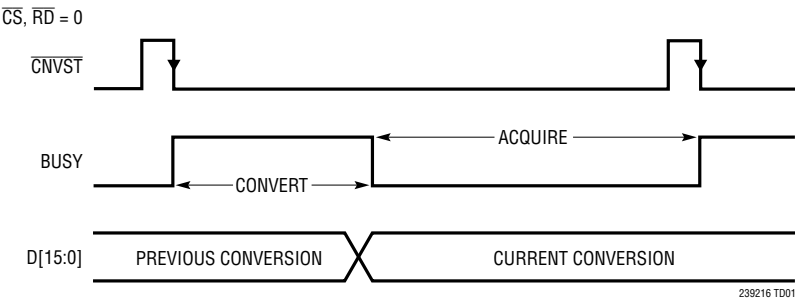
Conversion Timing Using the Parallel Interface
