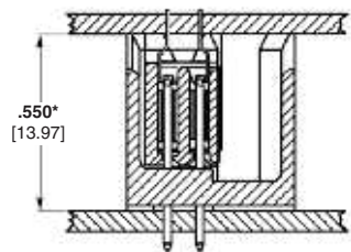
Figure 4 Double-Row, Two-Piece Receptacle and Two-Piece Shrouded Header *Mod II Shrouded Header Height is .440 [11.18] for a total stack height of .880 [22.38]
