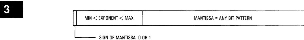
Figure 3-3. Format of Normalized Numbers
