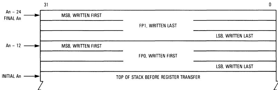
Figure 7-12. Transfer Multiple Floating-Point Data Register to Stack Example
