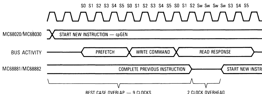
Figure 8-2. Best-Case Coprocessor Interface Overhead Timing
