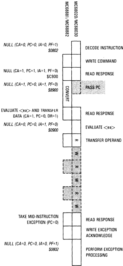
Figure 7-32. Take Mid-Instruction Exception Dialog — MC68882 General Concurrent Case
