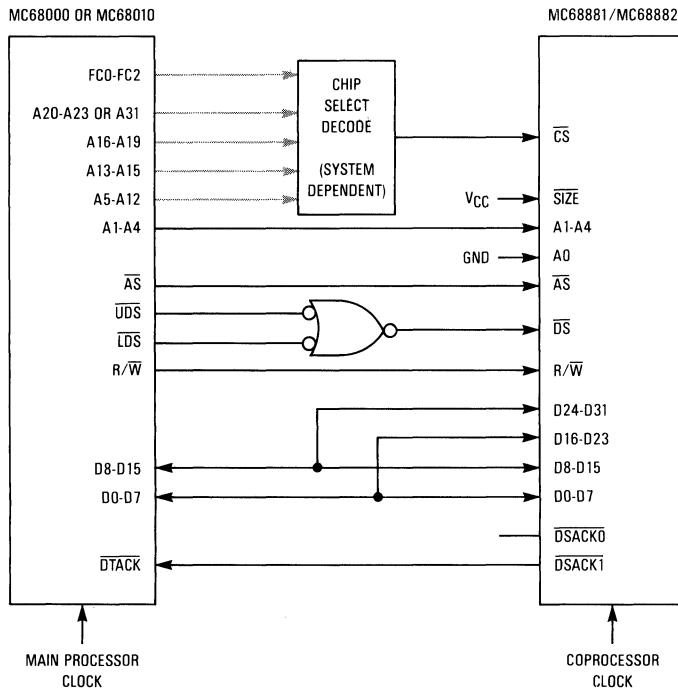
Figure 11-4. 16-Bit Data Bus Peripheral Processor Connection
