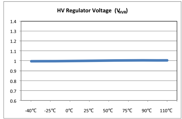
Figure 5. HV Regulator Voltage vs. Temperature
