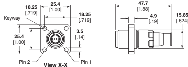
View X-X ODC 2 Fiber Socket Small Square to LC
