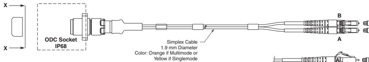
View X-X ODC 2 Fiber Socket Small Square to LC
