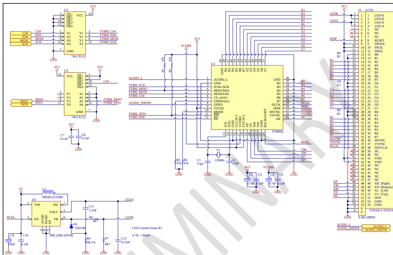
Figure 4-1 - VM800B35 ( 3.5" Version)
