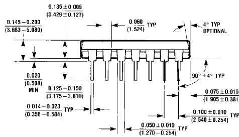
14-Lead Molded Dual-In-Line Package (N) Order Number DM74LS90N or DM74LS93N Package Number N14A
