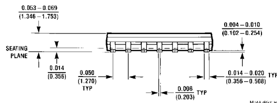
14-Lead Small Outline Molded Package (M) Order Number DM74LS90M or DM74LS93M Package Number M14A
