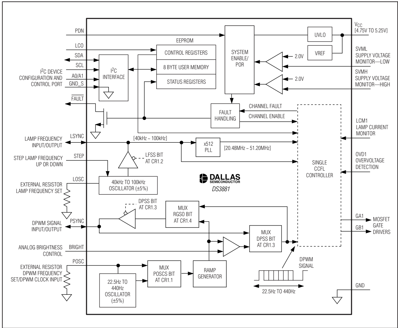
Figure 1. Functional Diagram
