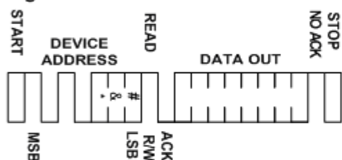
Figure 6: RANDOM READ (SDA INPUT/OUTPUT)
