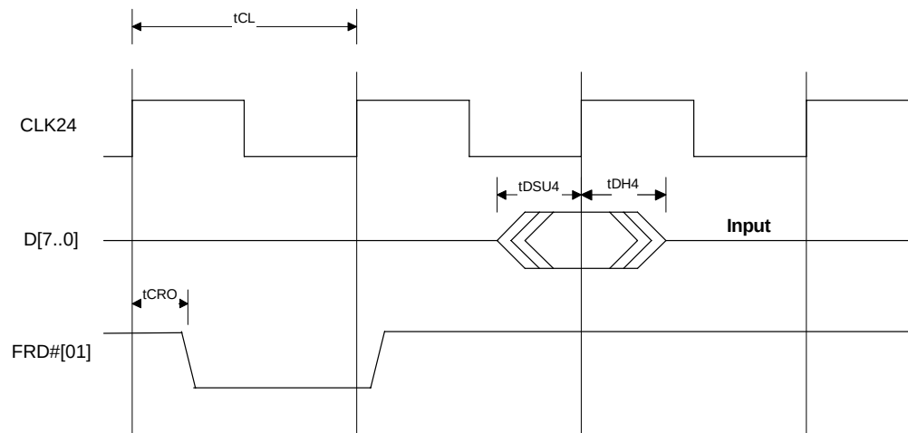
Figure 13-8. Fast Transfer Read Timing [Mode 01]
