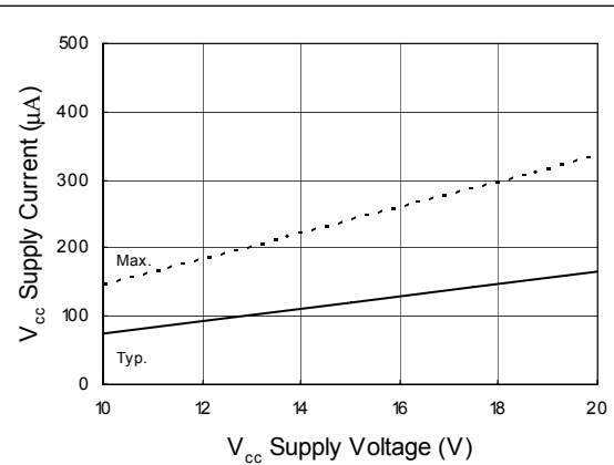
Figure 39B. IRS21171 V cc Supply Current vs. Supply Voltage
