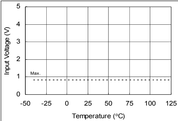
Figure 37A. IRS21171 Logic "0" Input Voltage vs. Temperature
