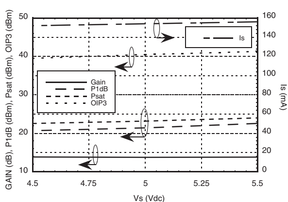
Gain, Power, OIP3 & Supply Current vs. Supply Voltage @ 850 MHz
