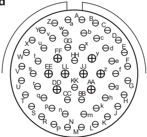
front face of pin inserts illustrated
