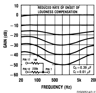
FIGURE 10. Loudness Compensated Volume Characteristic
