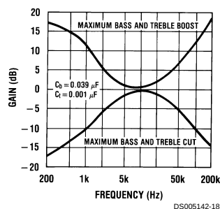
FIGURE 15. Tone Characteristic (Gain vs Frequency)
