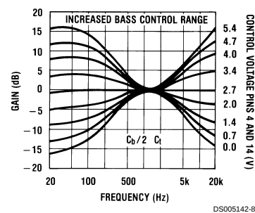
FIGURE 5. Tone Characteristic (Gain vs Frequency)
