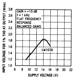
Input Signal Handling vs Supply Voltage
