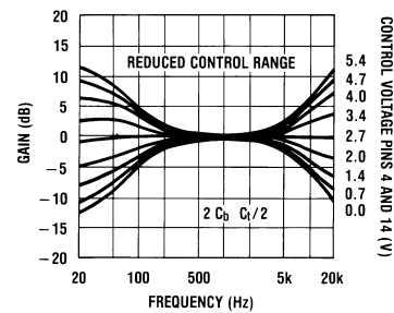
FIGURE 4. Tone Characteristic (Gain vs Frequency)
