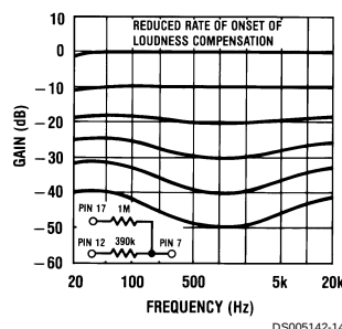
FIGURE 11. Loudness Compensated Volume Characteristic
