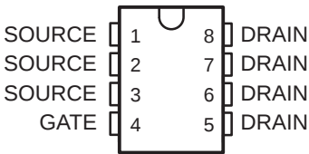
D PACKAGE
