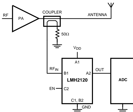
Figure 1. Typical Application
