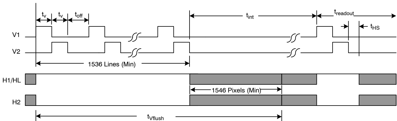
Figure 26. Flush Timing
