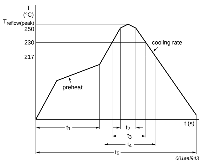
Fig 45. Pb-free solder reflow profile
