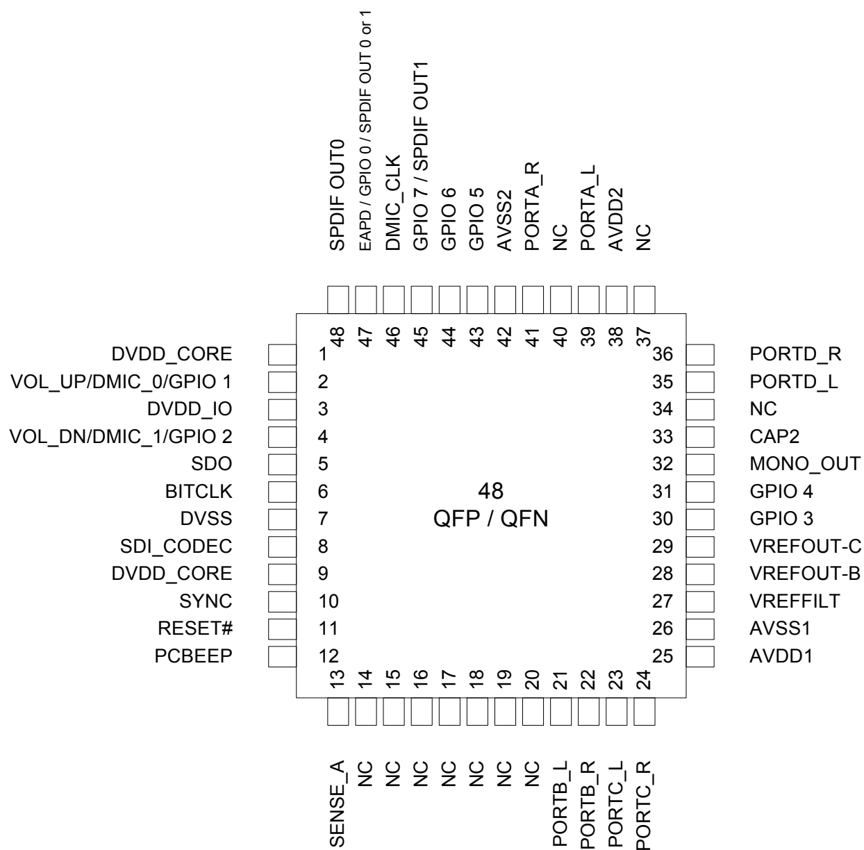
Figure 12. Pin Assignment
