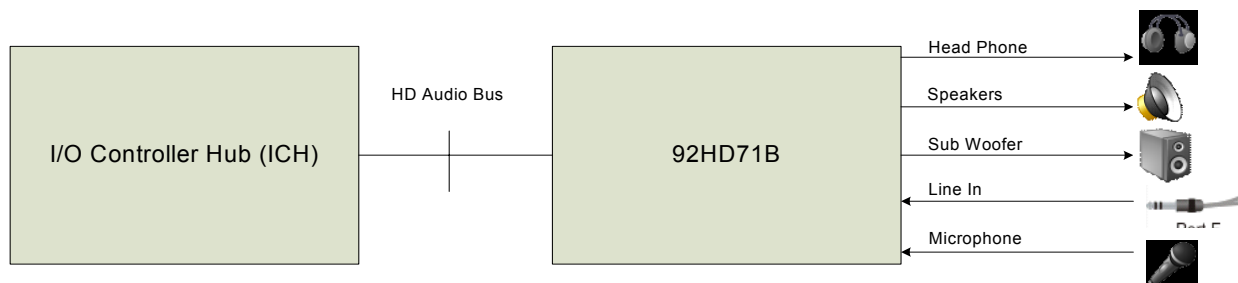
Figure 2. System Diagram
