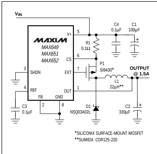
Figure 1. Test Circuit
