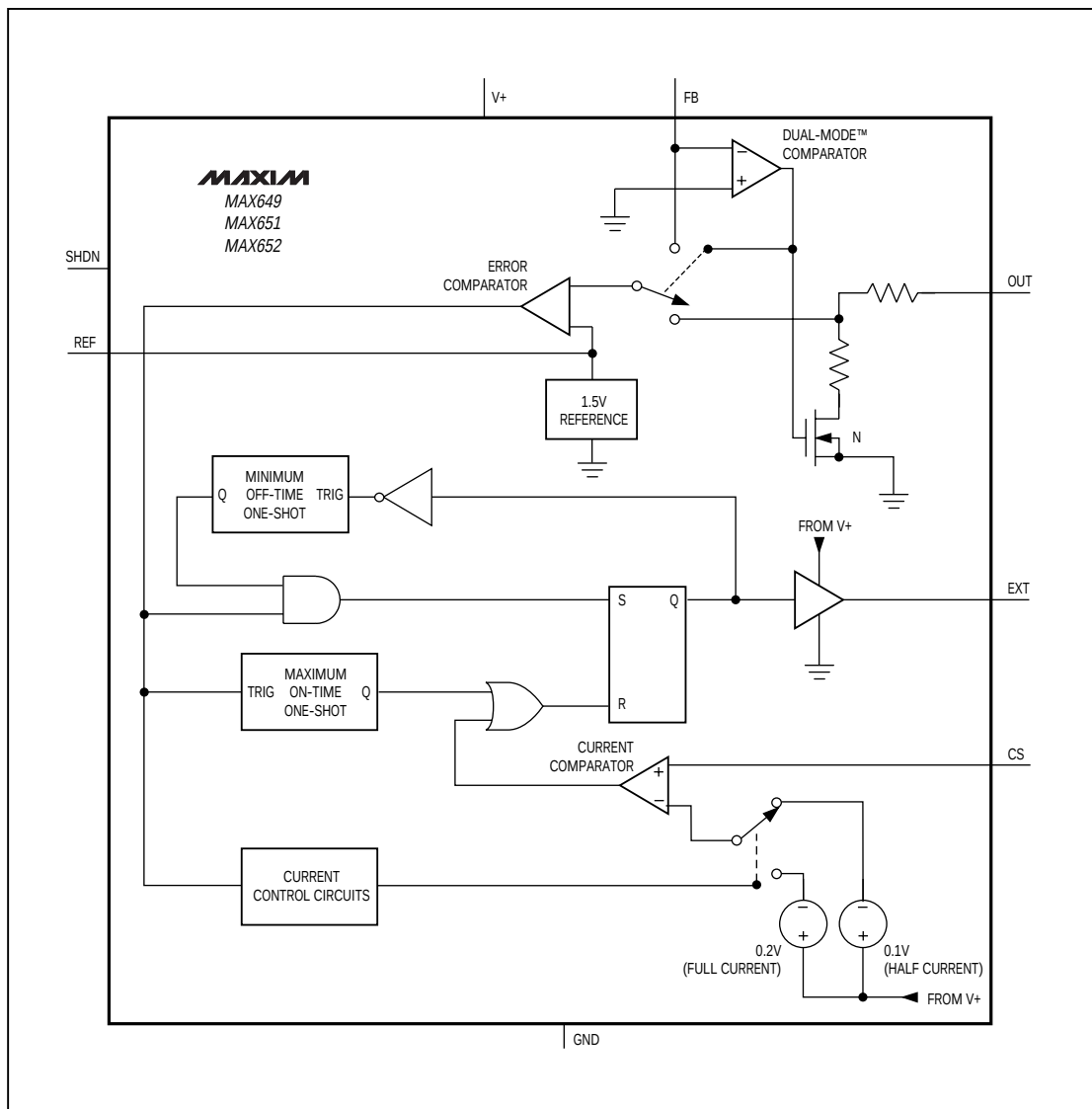
Figure 2. Block Diagram
