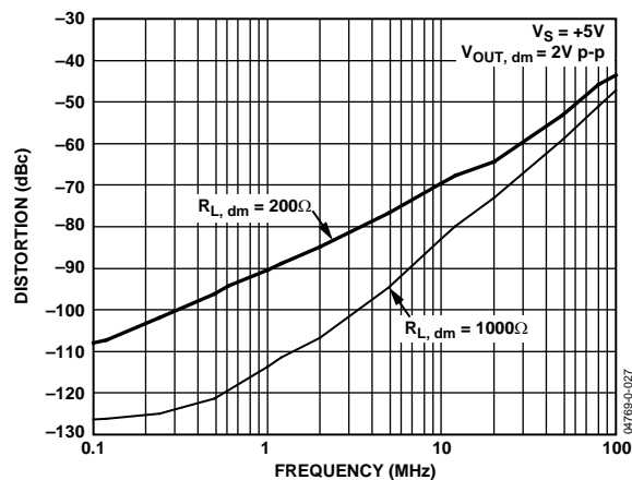
Figure 7. Second Harmonic Distortion at V_S = 5\text{ V} at Various Loads
