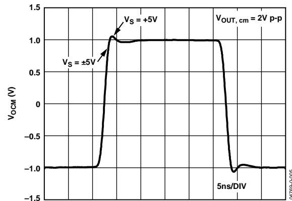
Figure 27. V_{OCM} Large Signal Transient Response for Various Power Supply Voltages
