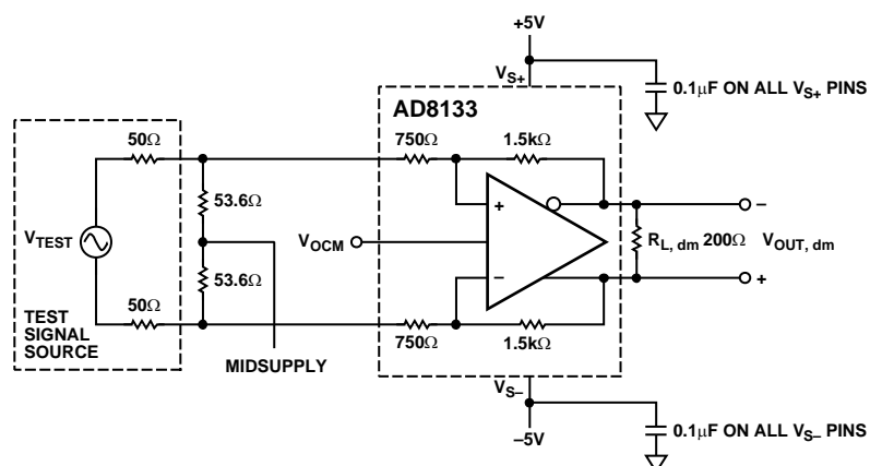
Figure 33. Basic Test Circuit
