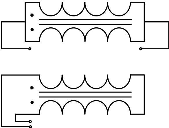
Differential Mode
