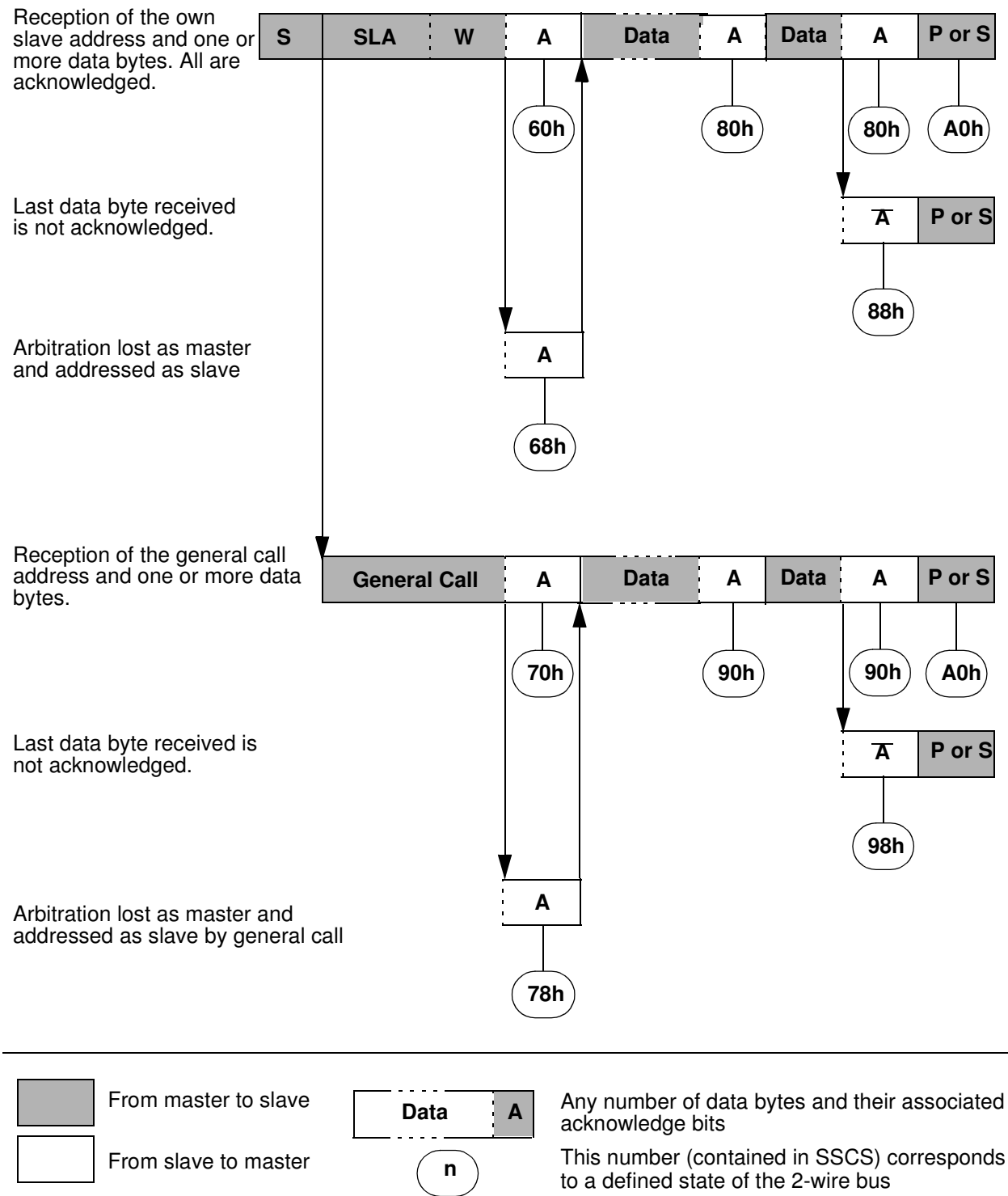
Figure 20-6. Format and State in the Slave Receiver Mode
