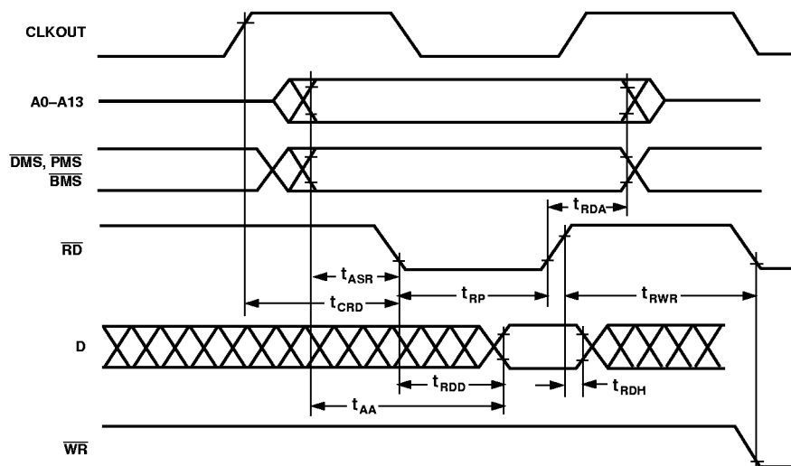
Figure 4. Memory Read
