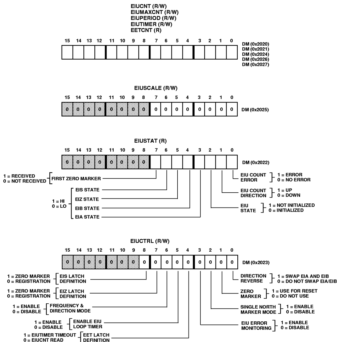
Figure 37. Structure of Registers of ADMC401
