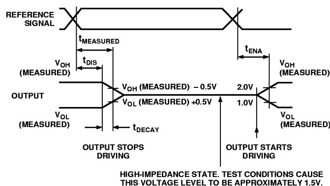
Figure 8. Output Enable/Disable
