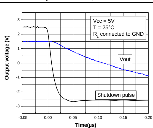
Figure 24. Turn-off time, V_{CC} = 5 V, Vout pulled down, T = 25^\circ\text{C}
