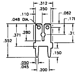
DUAL .110/.250 TAB
