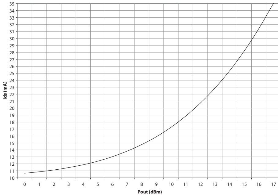
Figure 40. I_{ds} vs. P_{out} ( V_d = 5\text{V} )
