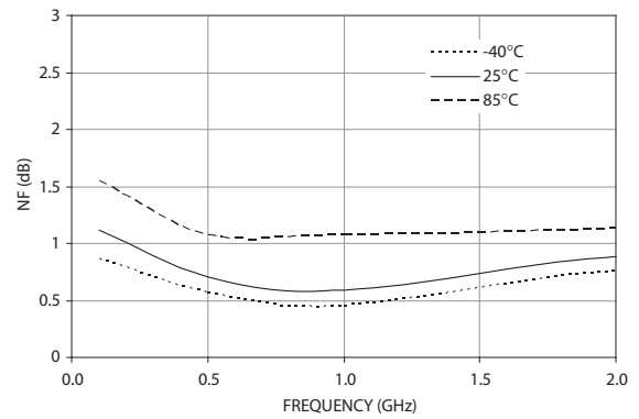
Figure 30. NF vs. Frequency (5V 15mA)
