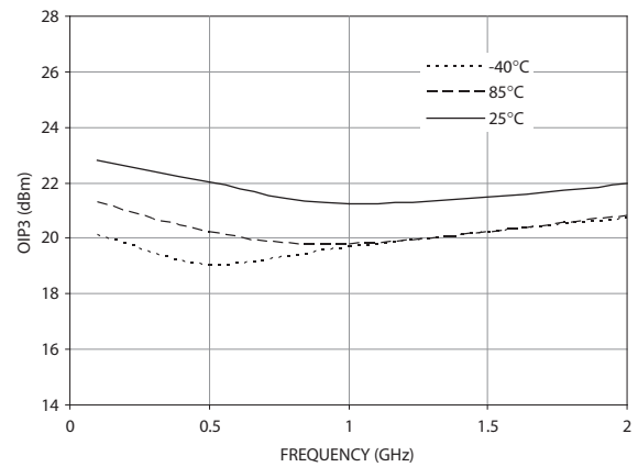
Figure 28. OIP3 vs. Frequency (5V 15mA)
