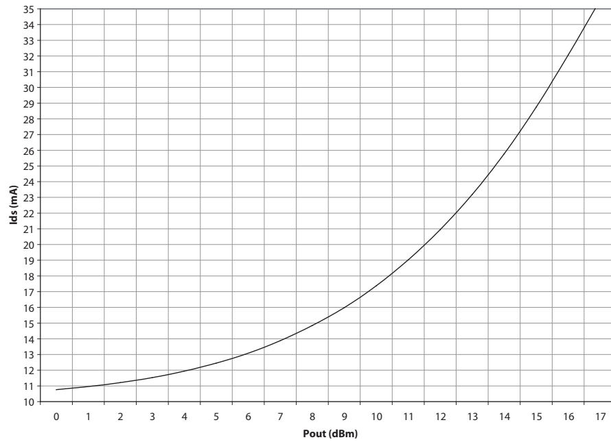
Figure 39. I_{ds} vs. P_{out} ( V_d = 3\text{V} )
