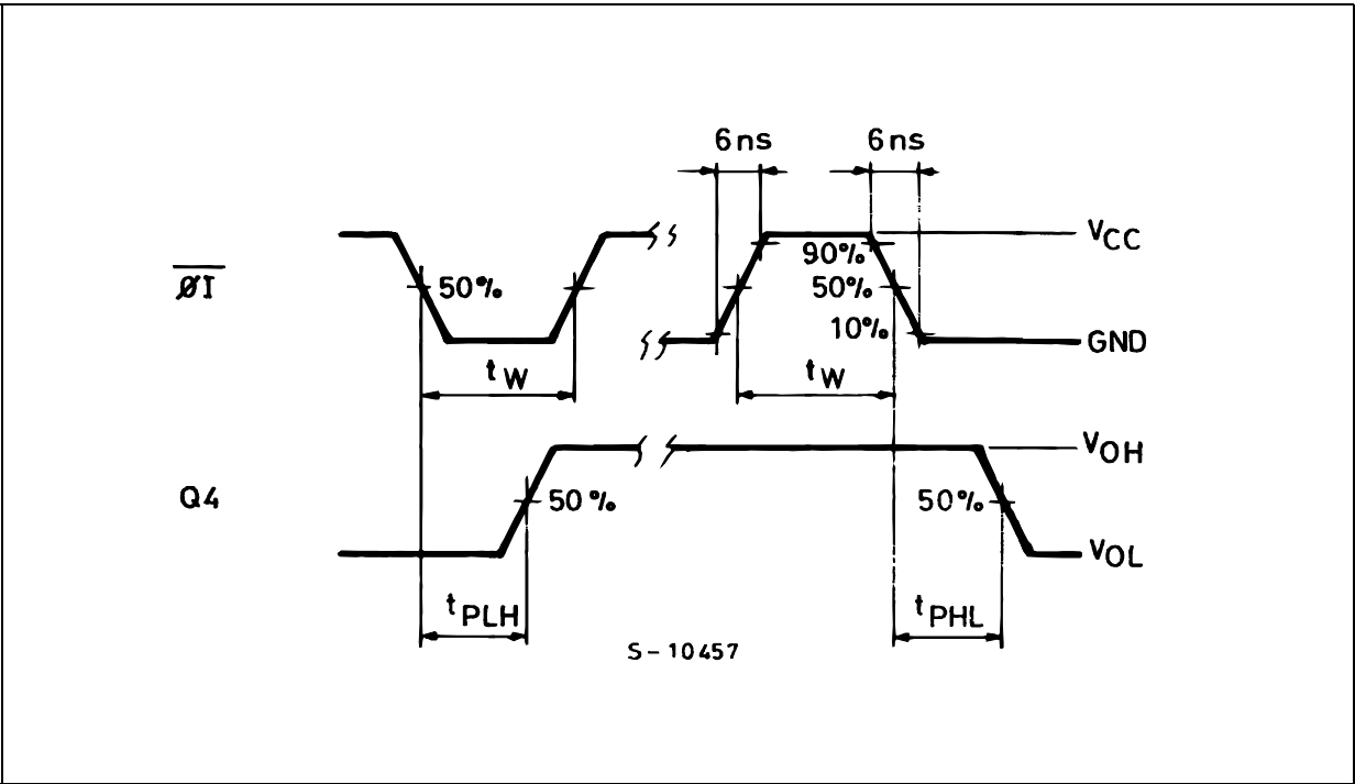
Figure 5: Waveform - Propagation Delay Times, Minimum Pulse Width ( \overline{\phi I} ) (f=1MHz; 50% duty cycle)
