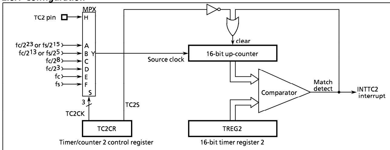
Figure 2-20. Timer/Counter 2
