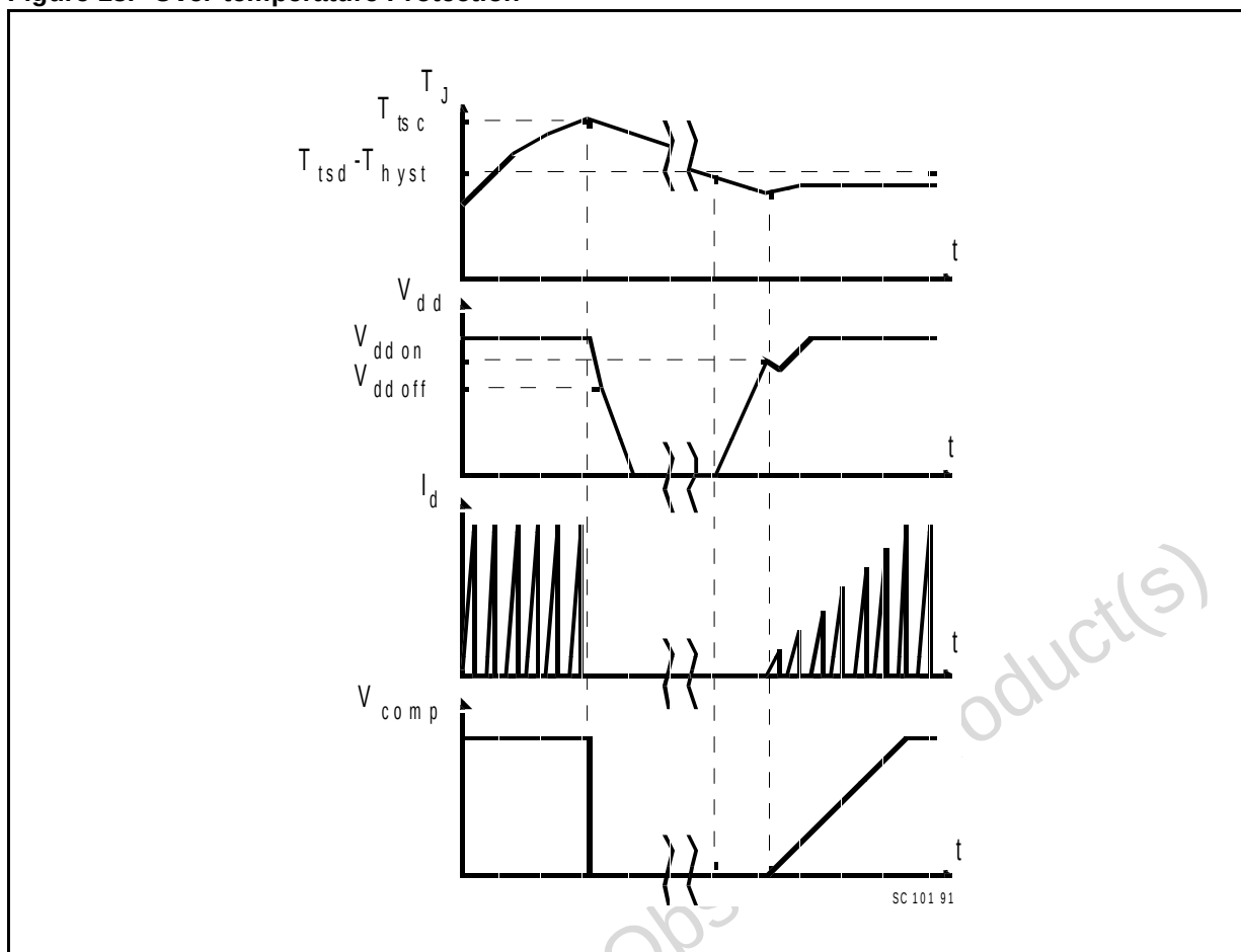
Figure 13. Over-temperature Protection
