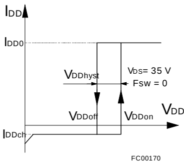
Figure 8. Shutdown Action
