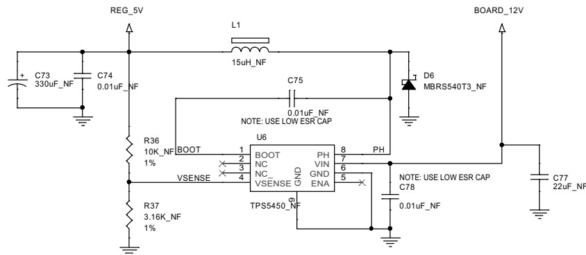
Figure 7-7. Reference Design 5
