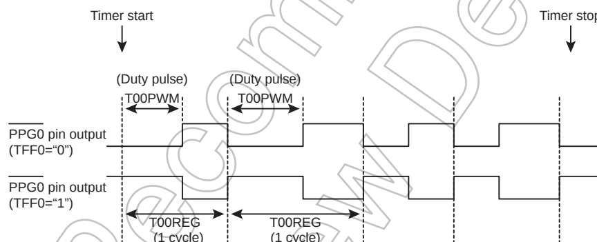
Figure 14-8 PPG0 Pulse Output
