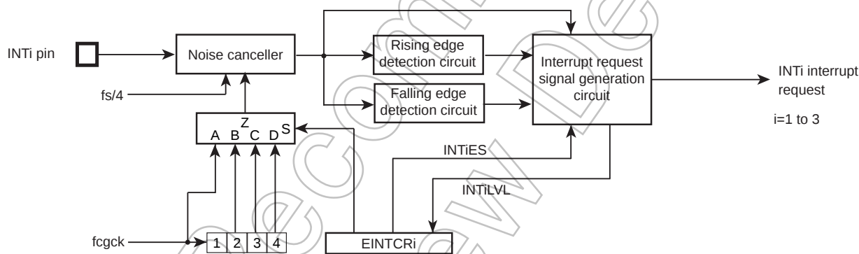
Figure 4-2 External Interrupts 1/2/3
