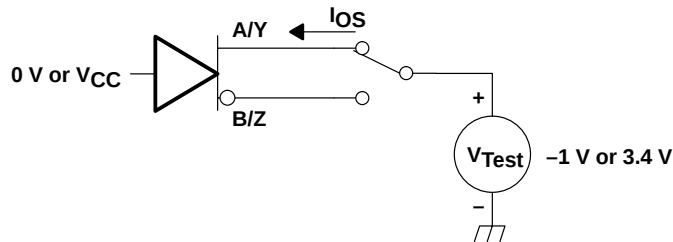
Figure 4. Driver Short-Circuit Test Circuit
