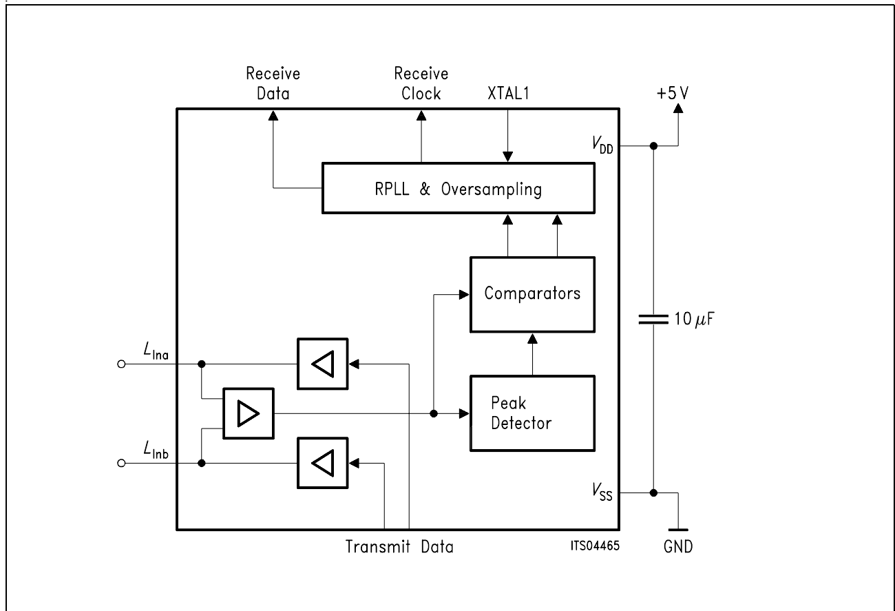
Figure 2-6 Transceiver Functional Blocks
