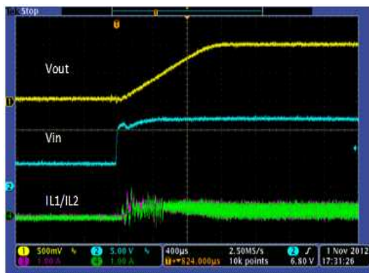
Figure 33. Current Share Mode Startup
