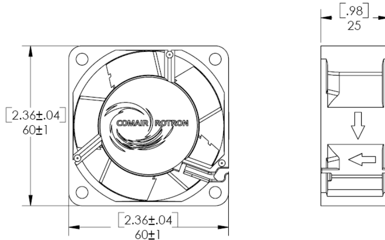
MECHANICAL DRAWING
