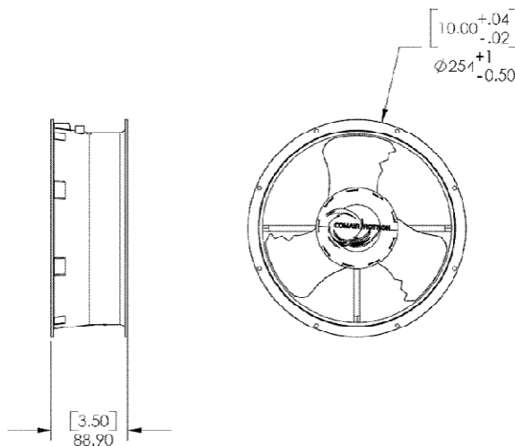
MECHANICAL DRAWING
