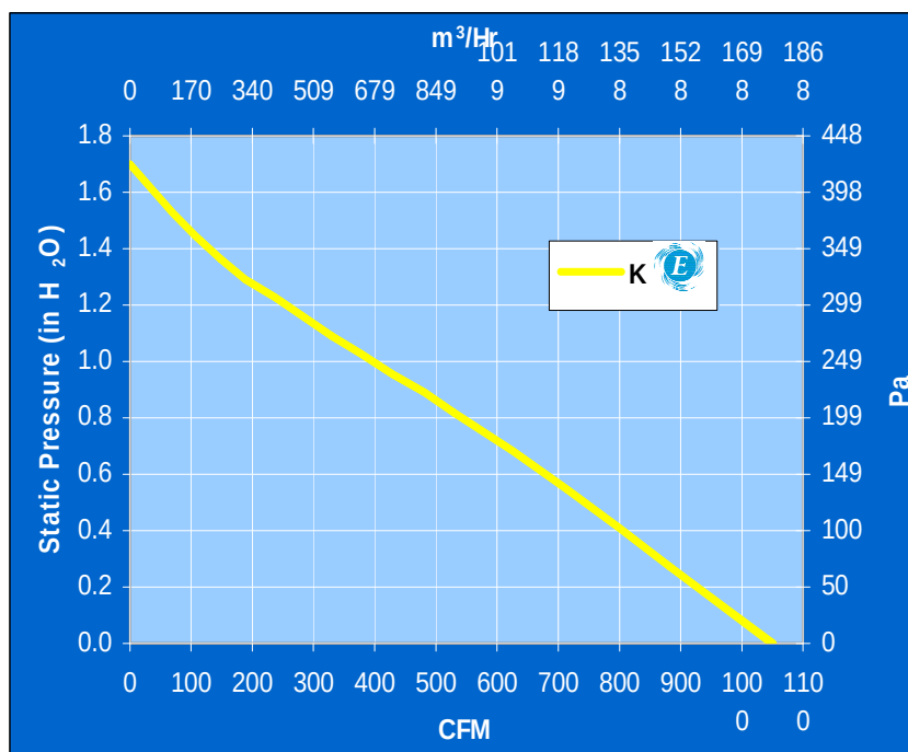
PERFORMANCE GRAPH
