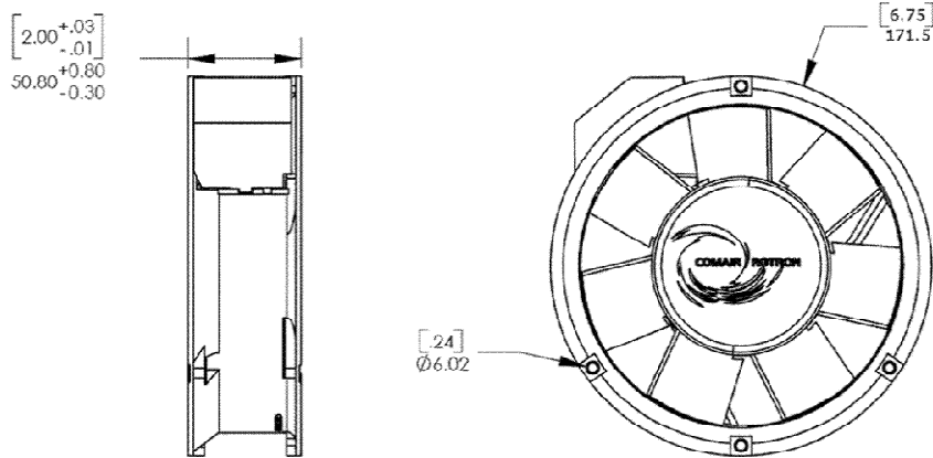
MECHANICAL DRAWING
