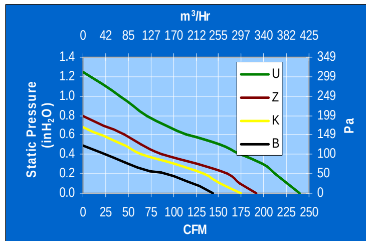
PERFORMANCE GRAPH
