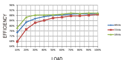
RSD-30H-12
