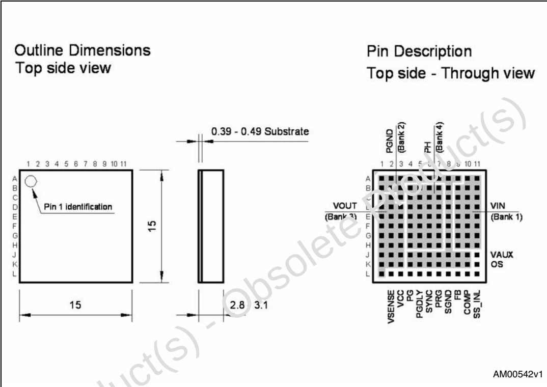
Figure 1. Pin connection
