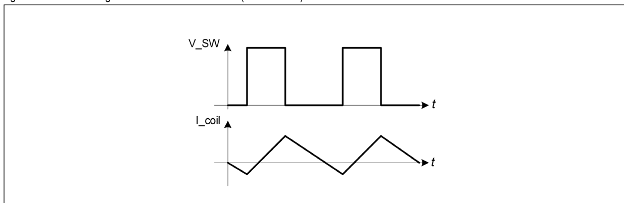
Figure 28. Switch voltage and coil current waveforms (MODE = low)
