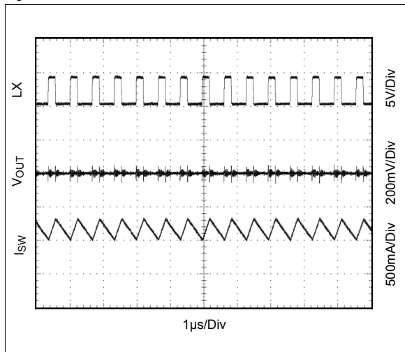
Figure 25. Continuous Current Mode
